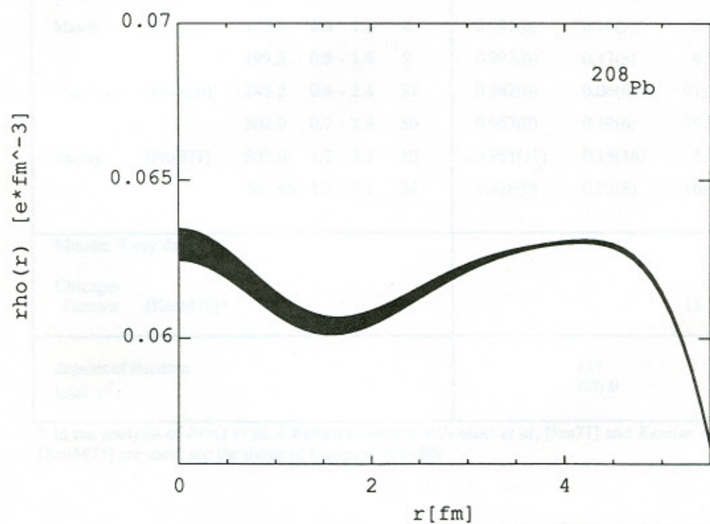
Figure 4.5. The charge density distribution determined by the reference fit of this work.
